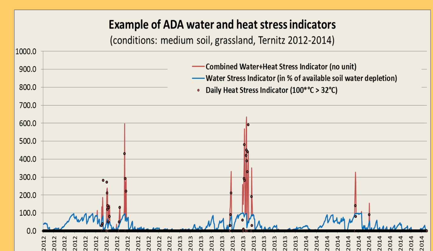
Fig.3. Time series of ADA crop drought/heat indicators.
